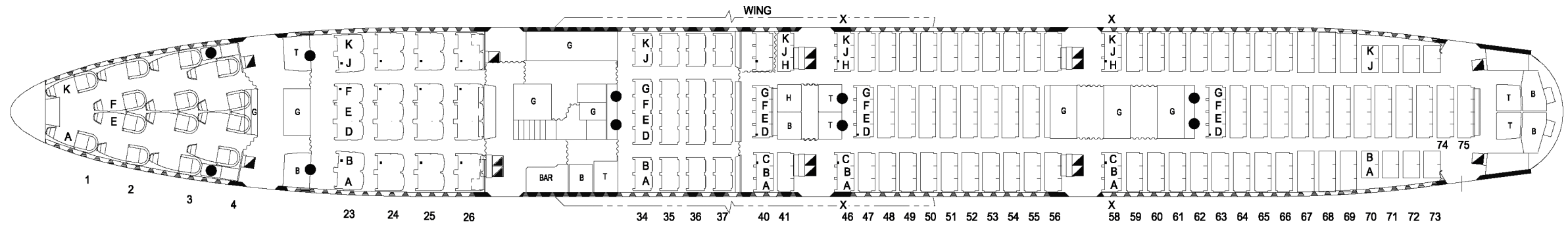
ZONE C PREMIUM ECONOMY CLASS 32 SEATS ECONOMY CLASS 13 SEATS (+3 CREW REST)
