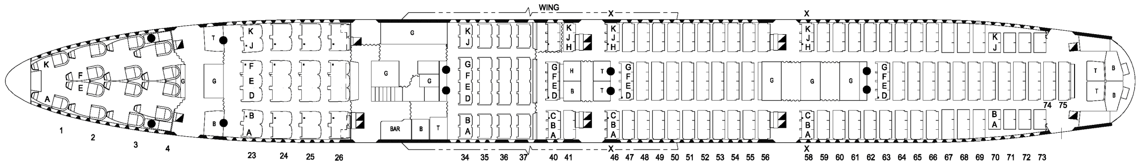
ZONE A LUXURY FIRST CLASS 14 SEATS ZONE B BUSINESS CLASS 28 SEATS ZONE C PREMIUM ECONOMY CLASS 32 SEATS ECONOMY CLASS 13 SEATS (+3 CREW REST) ZONE D ECONOMY CLASS 102 SEATS ZONE E ECONOMY CLASS 140 SEATS
